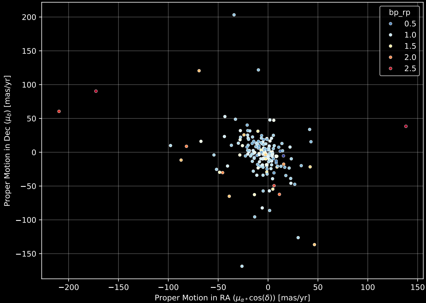
APOGEE DR17 Field: [074+45_MGA] Proper Motion Diagram (n= 189)
