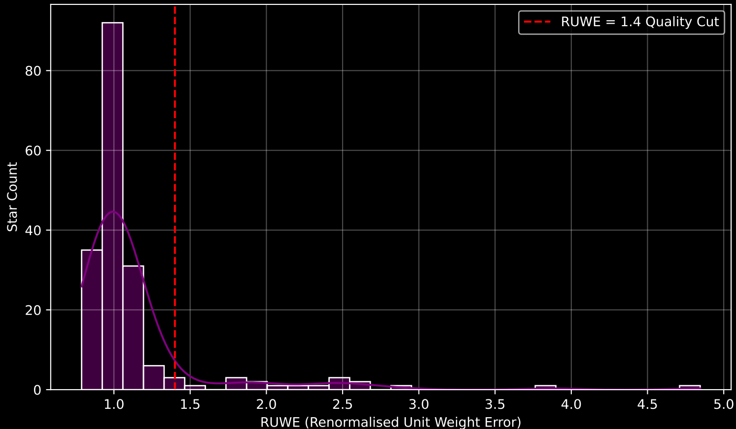
GAPOGEE DR17 Field [074+45_MGA] RUWE Distribution (n= 184)
