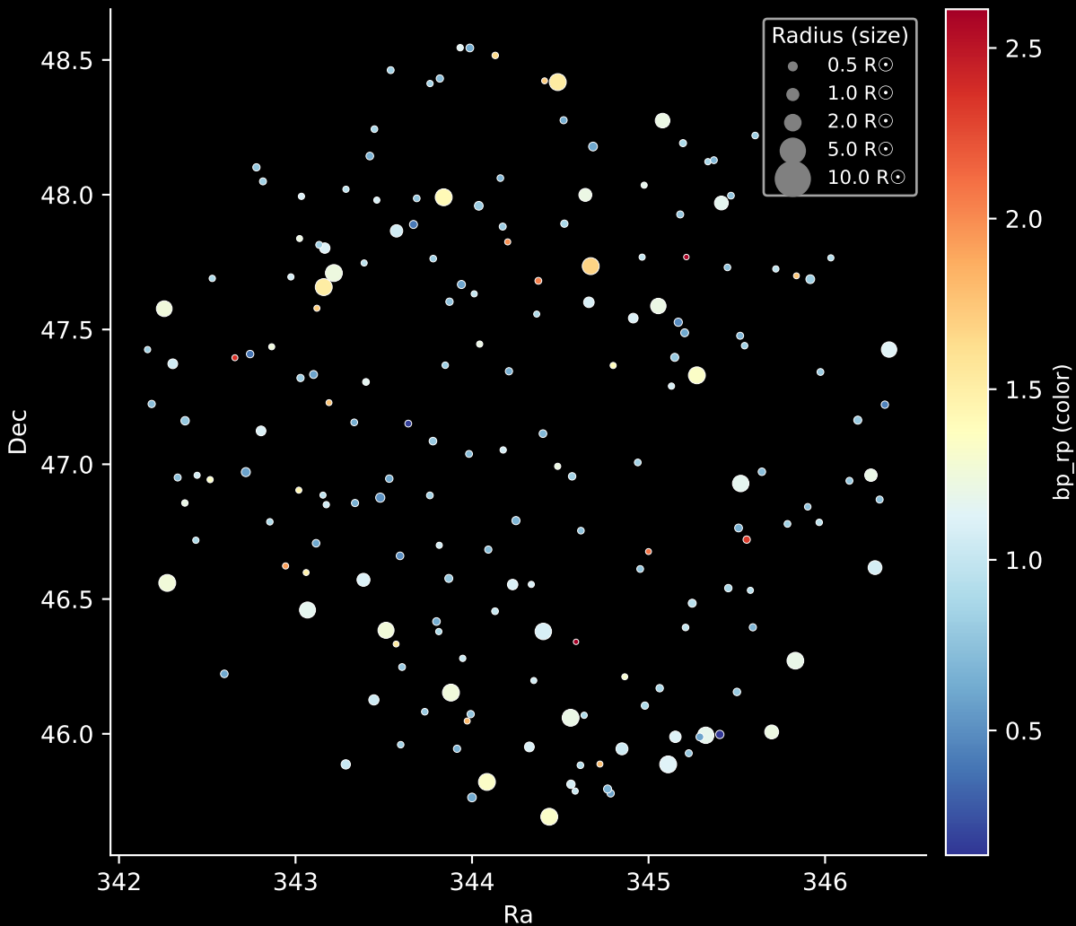
APOGEE DR17 Field: [074+45_MGA] Stars: 189
