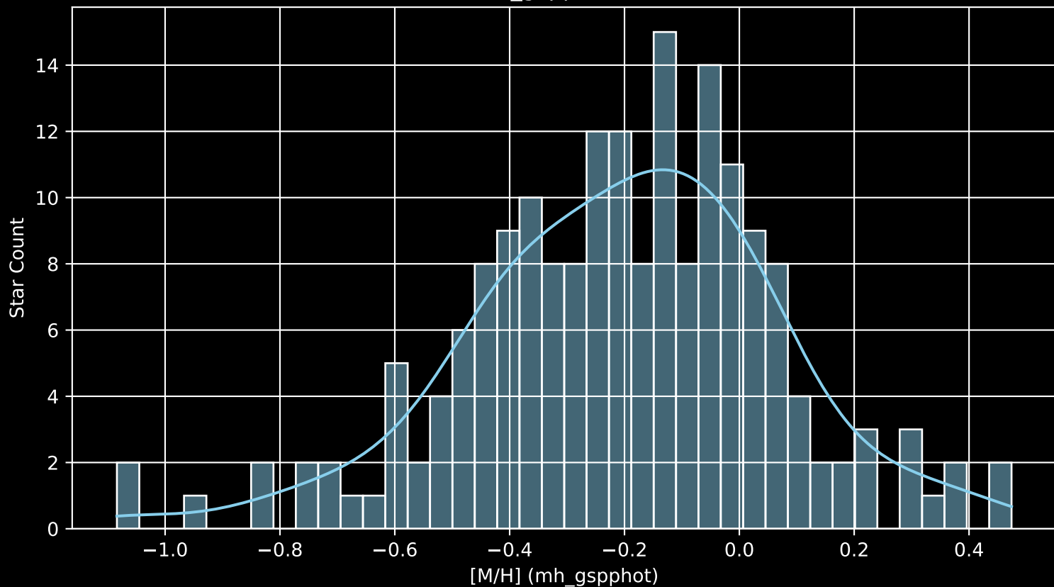
APOGEE DR17 Field: [074+45_MGA [M/H] (mh_gspphot) (n= 187)
