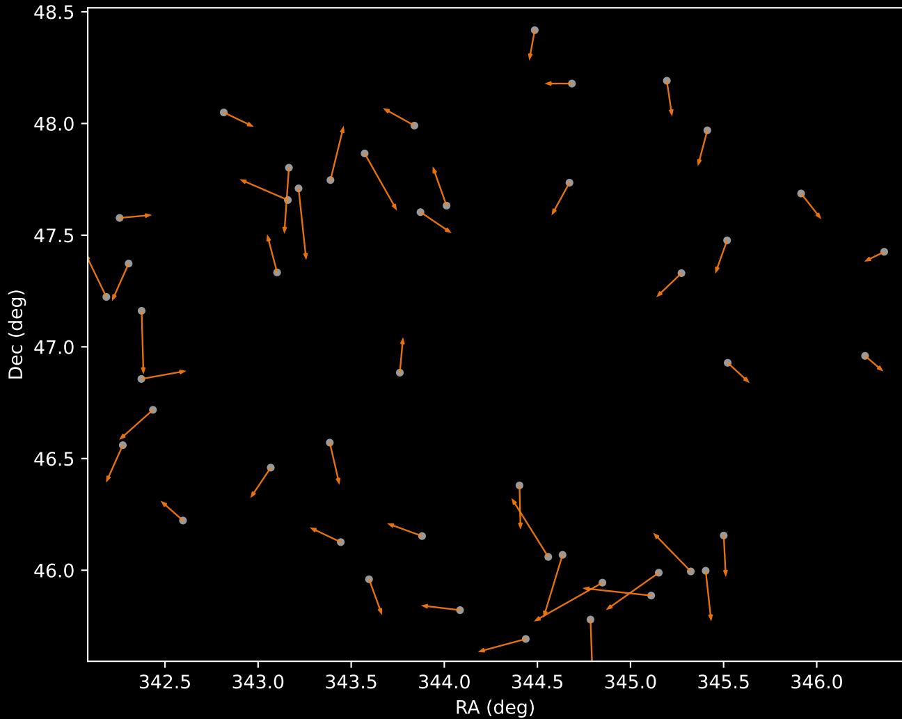
APOGEE DR17 Cluster 2 Proper Motion Vectors (n=47)
