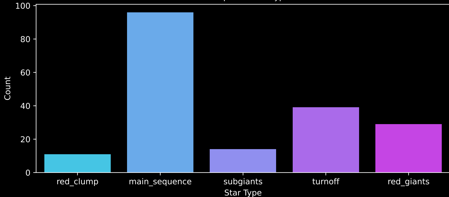
APOGEE DR17 Field: [074+45_MGA] Count plot of Star Type
