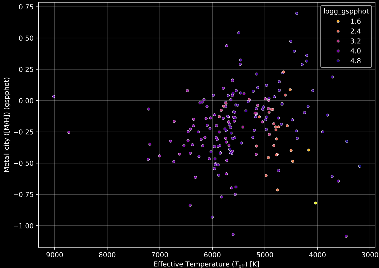
APOGEE DR17 Field: [074+45_MGA] Stellar Population Parameters (n= 189)
