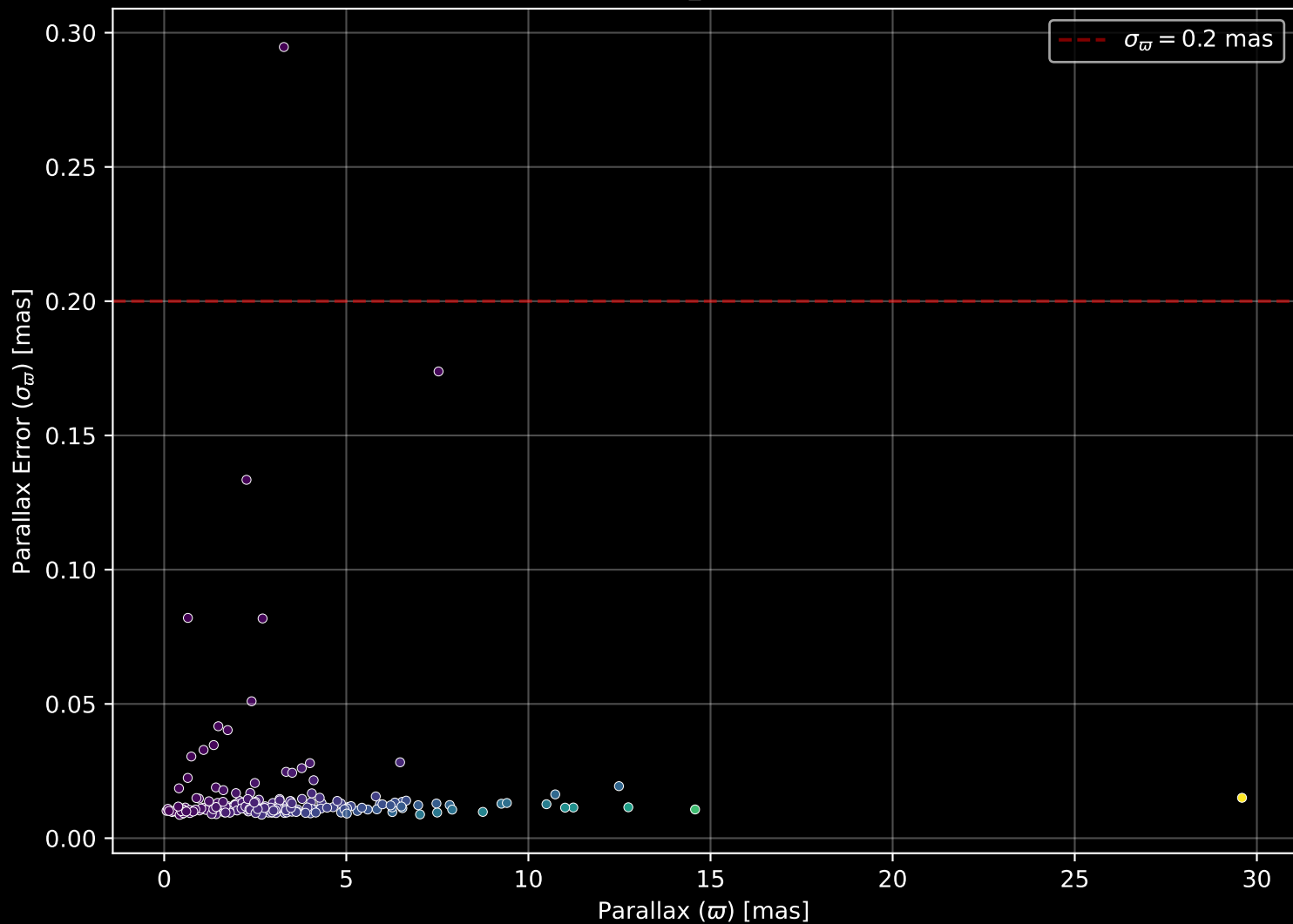
APOGEE DR17 Field: [074+45_MGA] Parallax Quality (n= 189)
